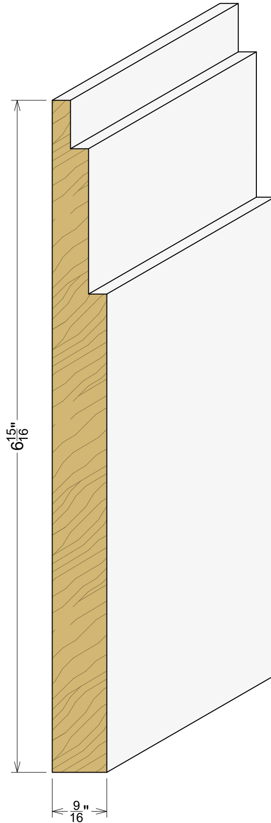
AP 4434 9/16"x 6 15/16"
