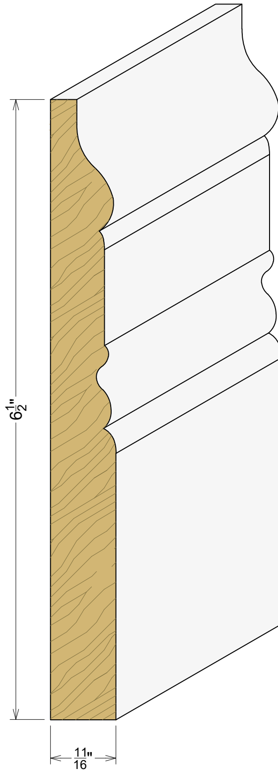
AP 4454 1 1/16" x 6 1/2"
