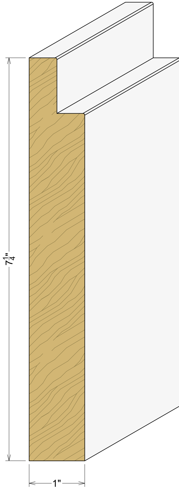
AP 4455 1"x 7 1/4"
