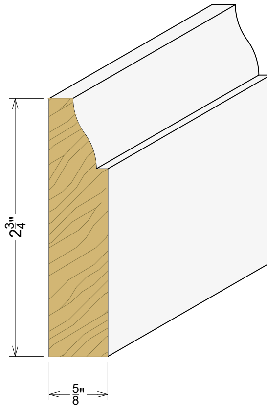
AP 4459 5/8"x 2 3/4"
