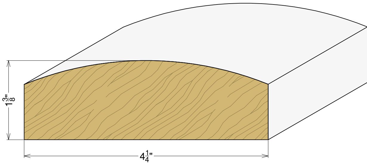
AP 5010 1-3/8" x 4-1/4"
