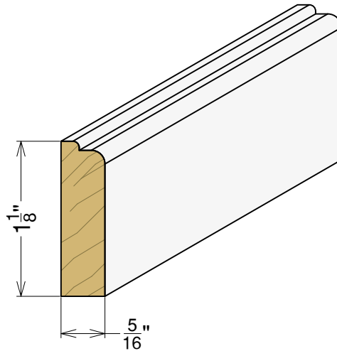
AP 5011 5/16" x 1-1/8"
