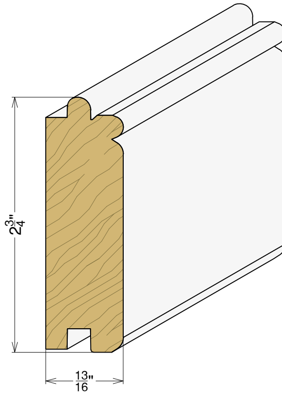
AP 5033 13/16" x 2-3/4"
