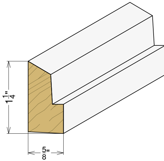
AP 5060 5/8" x 1-1/4"
