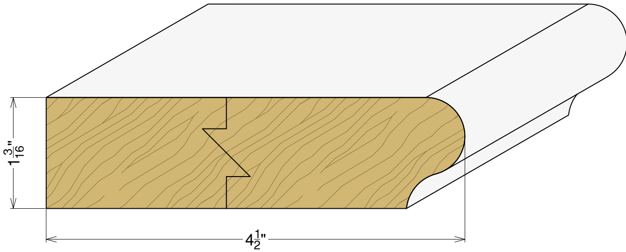
AP 5061 1-3/16" x up to 9-1/4"
