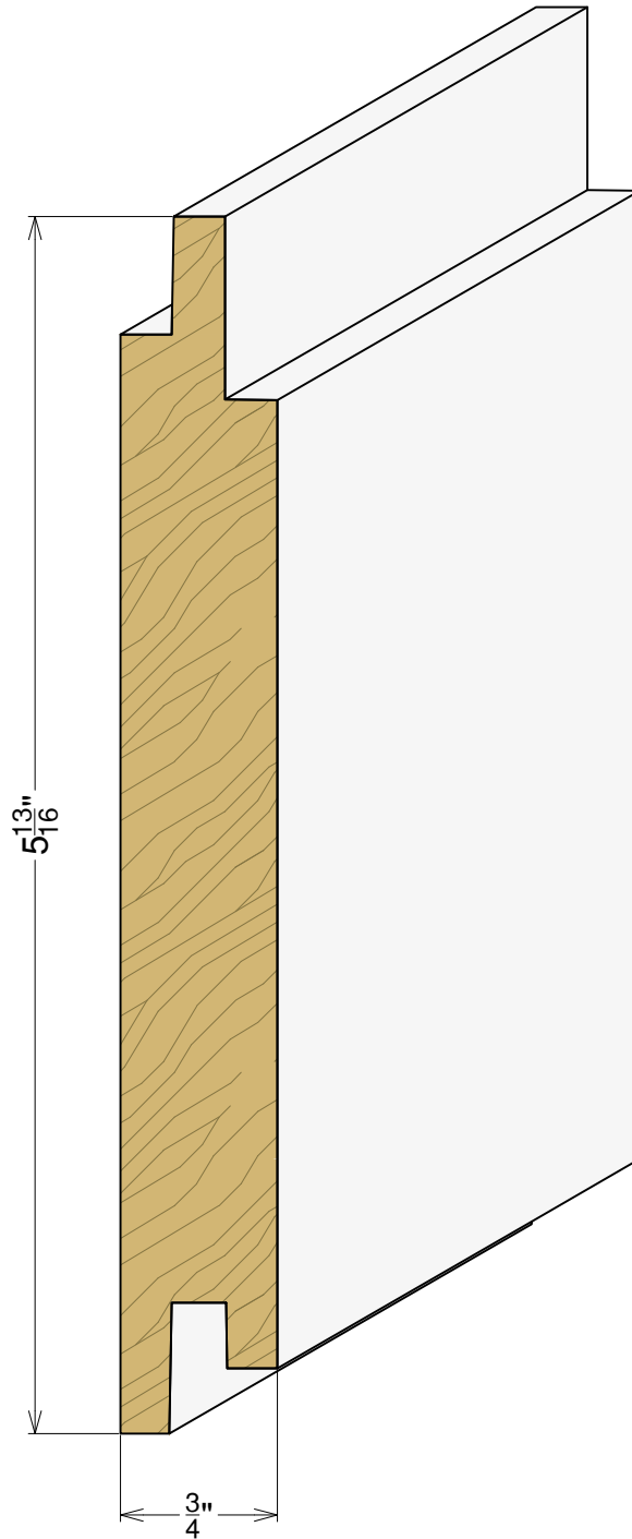
AP 5074 3/4" x 5-13/16"
