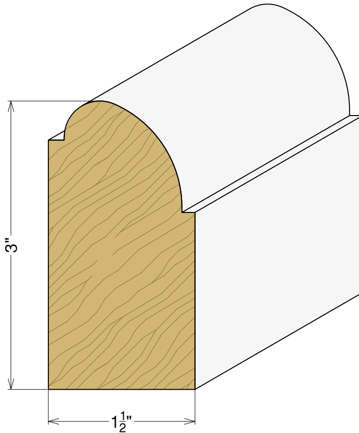
AP 5075 1-1/2" x 3"
