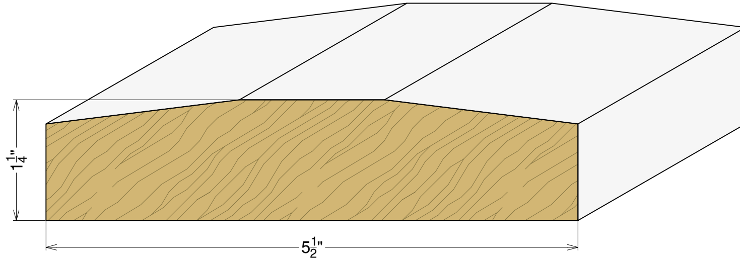
AP 5104 1-1/4" x 5-1/2"
