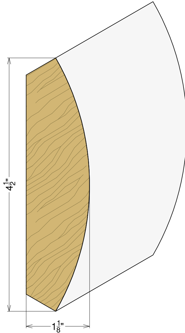
AP 5123 1-1/8" x 4-1/2"
