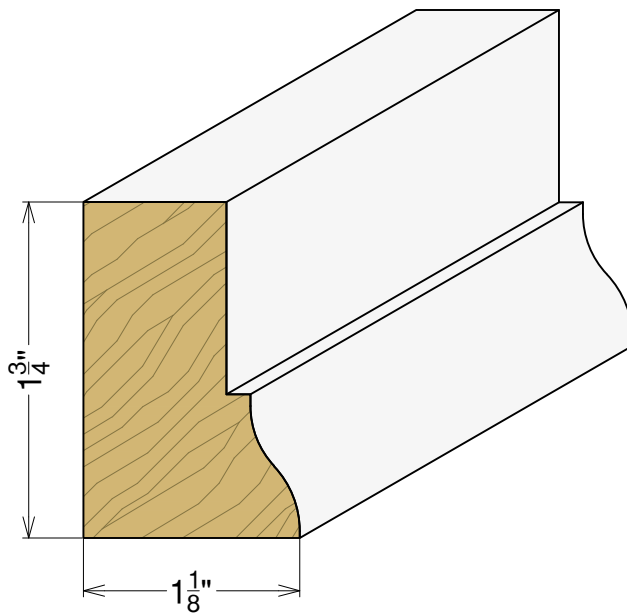
AP 5142 1-1/8" x 1-3/4"
