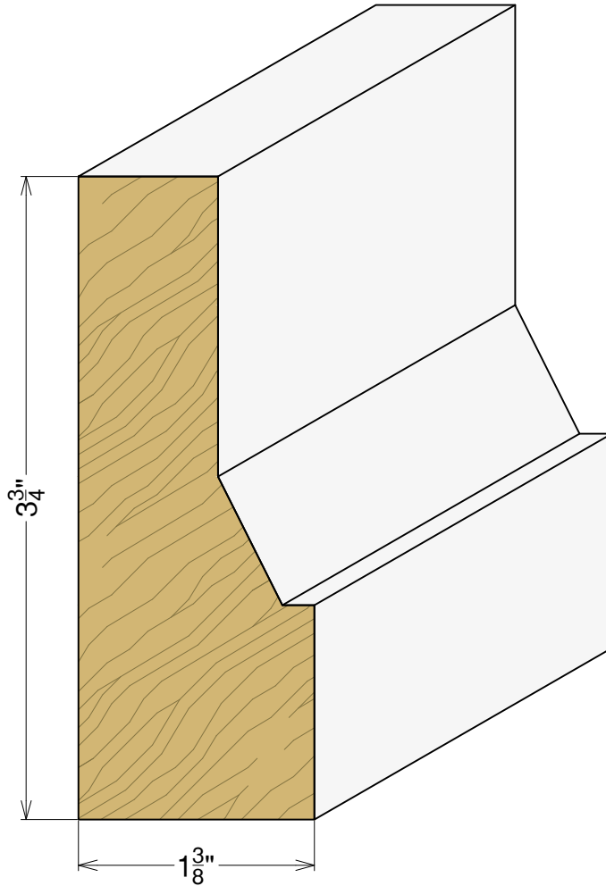
AP 5162 1-3/8" x 3-3/4"
