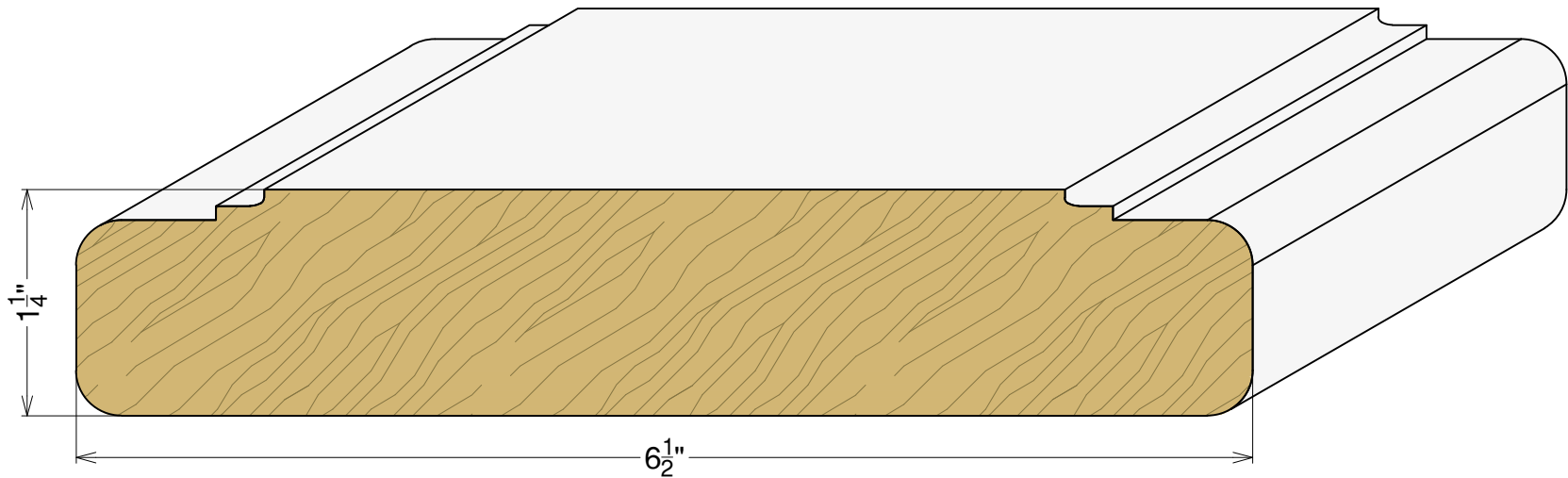
AP 5165 1-1/4" x 6-1/2"
