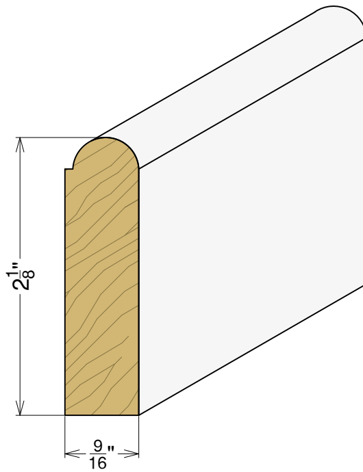
AP 5167 9/16" x 2-1/8"
