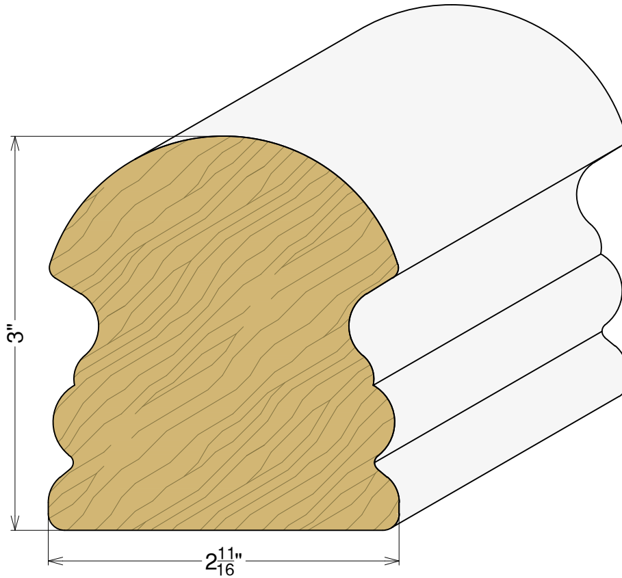
AP 5188 3" x 2-11/16"
