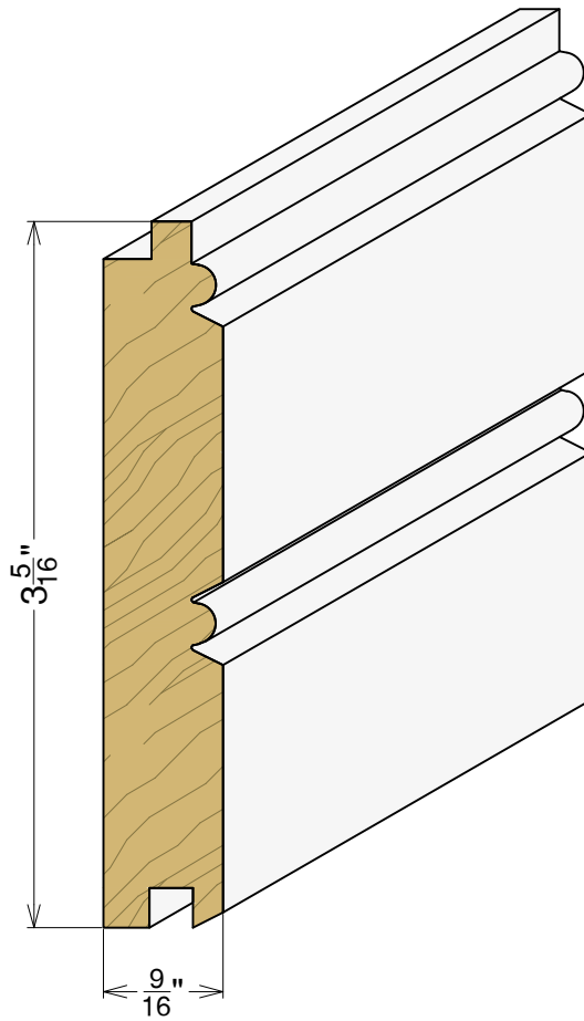
AP 5189 9/16" x 3-5/16"
