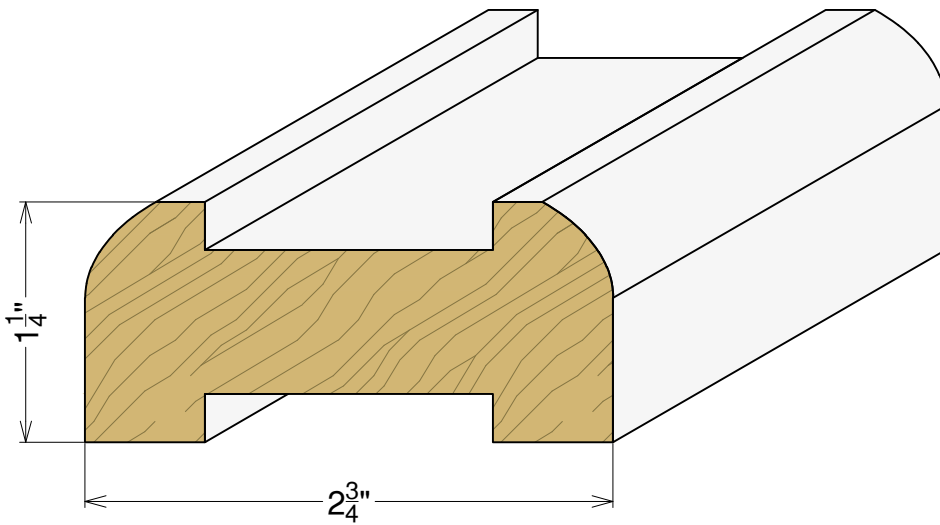
AP 5196 1-1/4" x 2-3/4"
