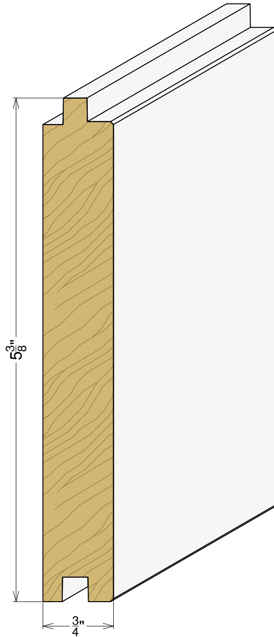
AP 5219 3/4" x 5-3/8"
