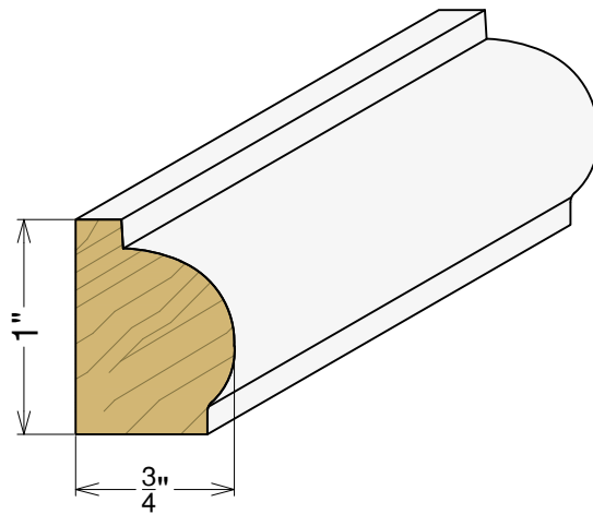
AP 5266 3/4" x 1"
