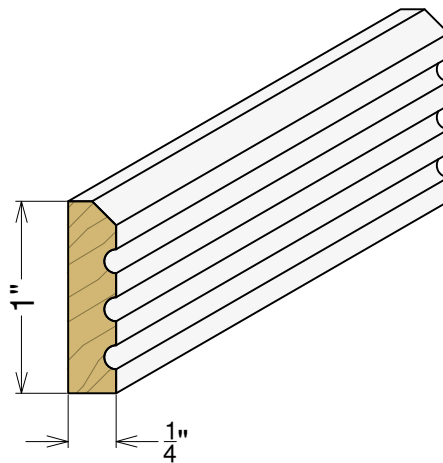
AP 5303 1/4" x 1"
