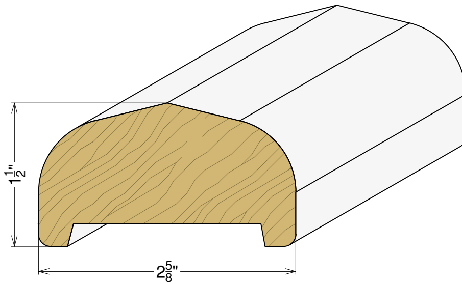
AP 5320 1-1/2" x 2-5/8"
