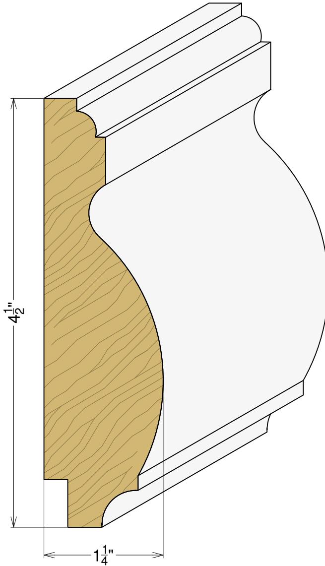
AP 5332 1-1/4" x 4-1/2"
