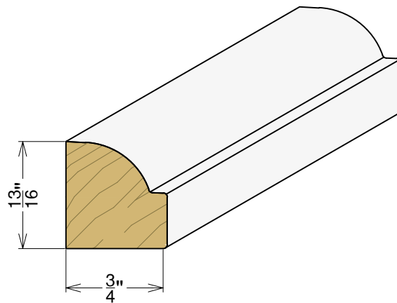
AP 5404 3/4" x 13/16"
