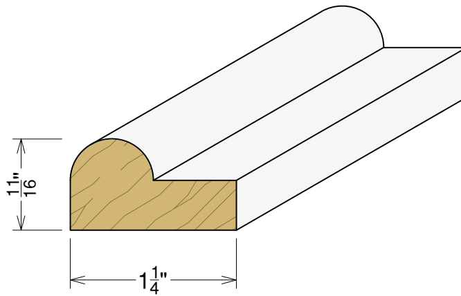
AP 5485 1 1/16" x 1 1/4"
