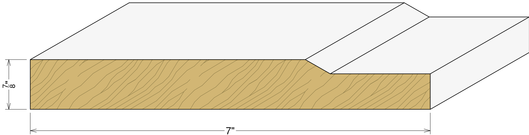
AP 5488 7/8"x 7"
