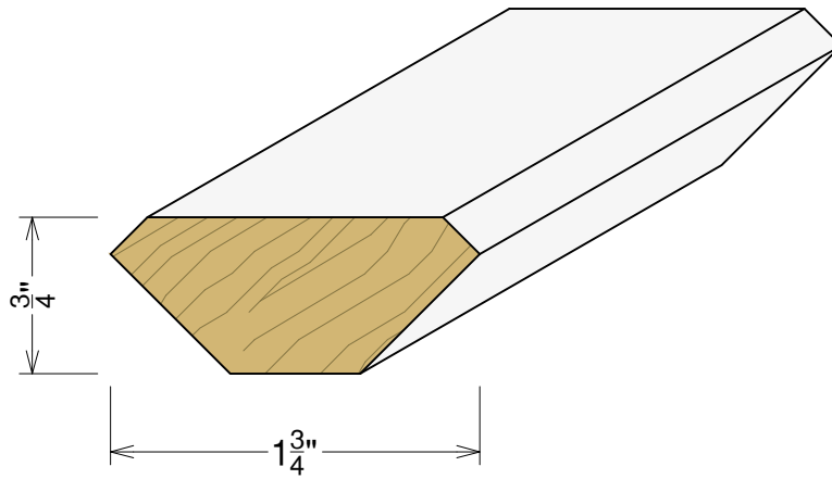
AP 5490 3/4" x 1 3/4"
