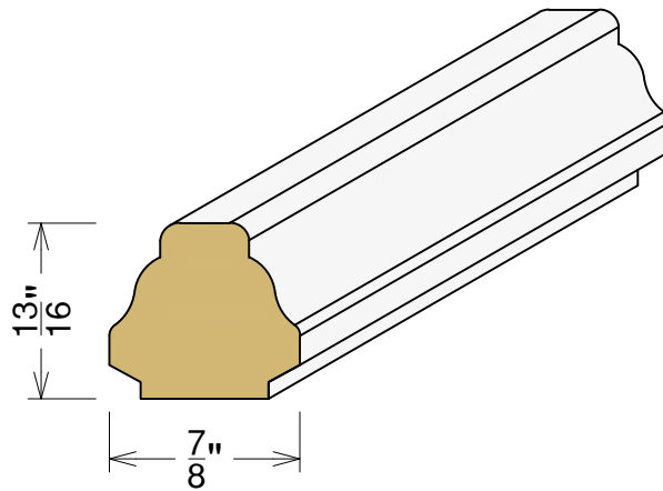
AP 5494 13/16"x 7/8"
