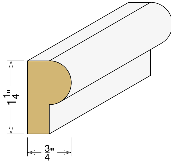
AP 5495 3/4"x 1 1/4"
