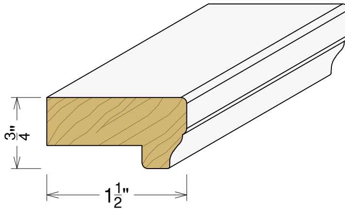
AP 5500 3/4"x 1 1/2"
