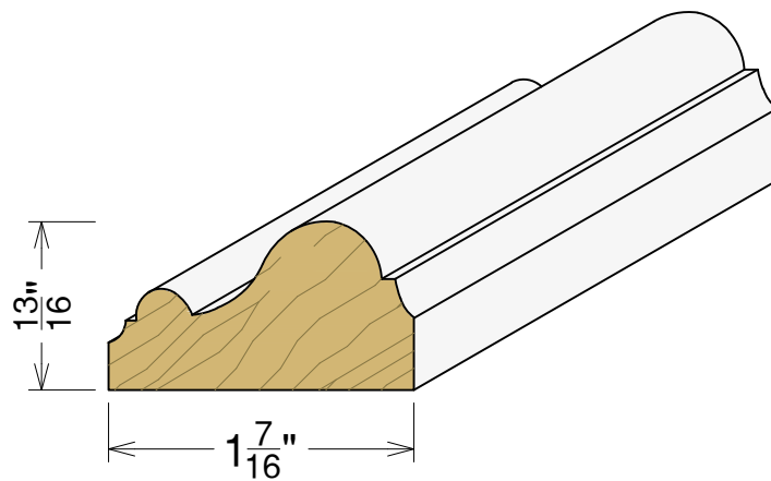
AP 5504 13/16"x 1 7/16"
