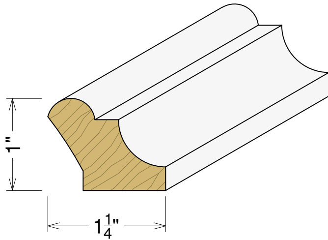
AP 5517 1"x 1 1/4"
