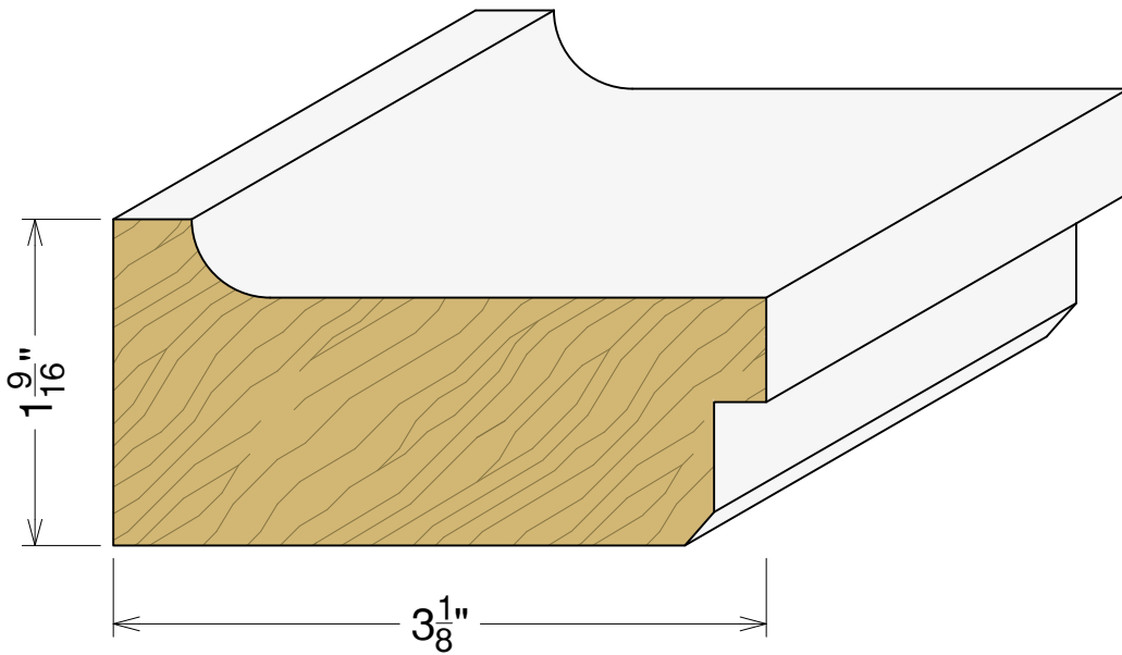
AP 5518 1 9/16"x 3 1/8"
