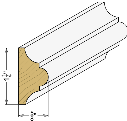
AP 6010 5/8" x 1-1/4"
