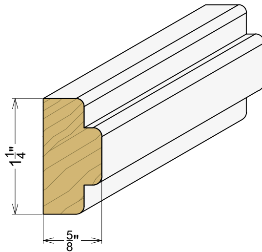
AP 6021 5/8" x 1-1/4"
