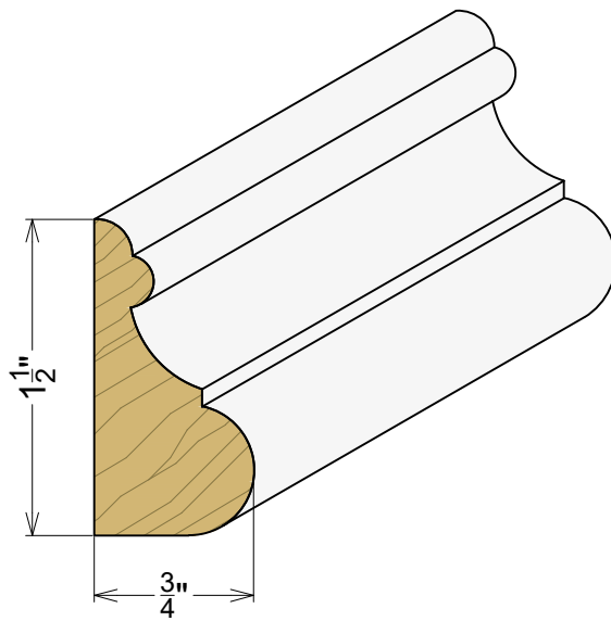
AP 6025 3/4" x 1-1/2"
