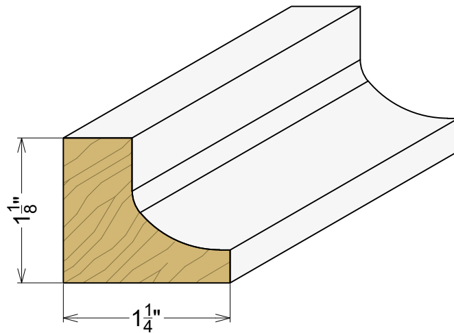
AP 6027 1-1/8" x 1-1/4"
