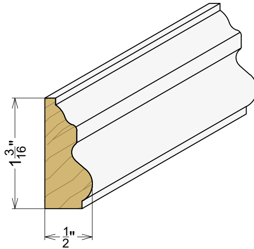
AP 6038 1/2" x 1-3/16"
