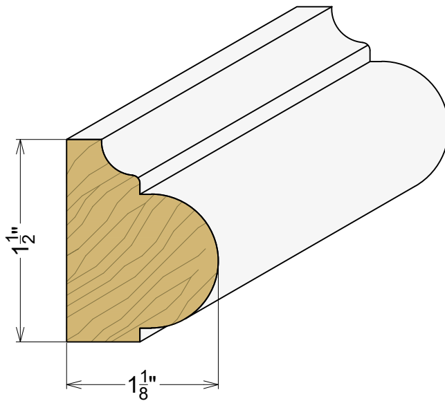
AP 6062 1-1/8" x 1-1/2"
