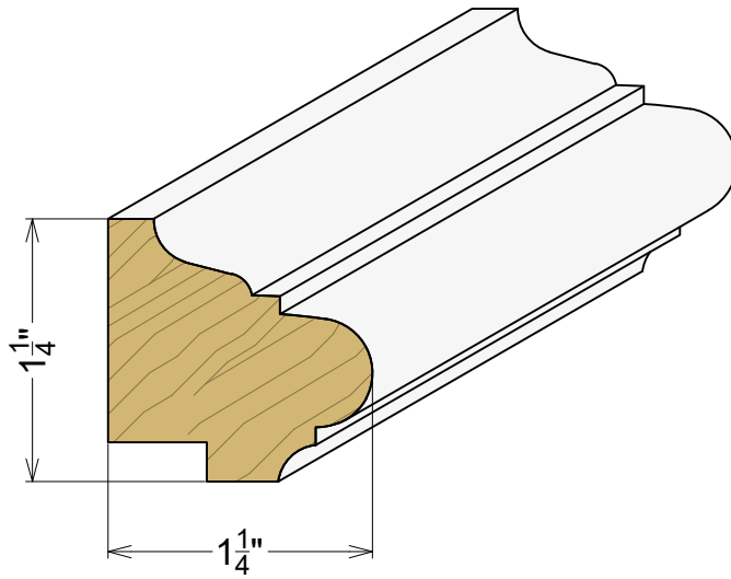
AP 6087 1-1/4" x 1-1/4"
