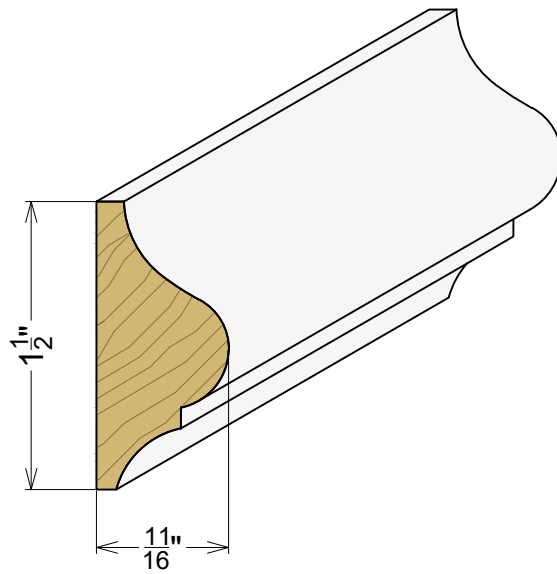
AP 6097 11/16" x 1-1/2"
