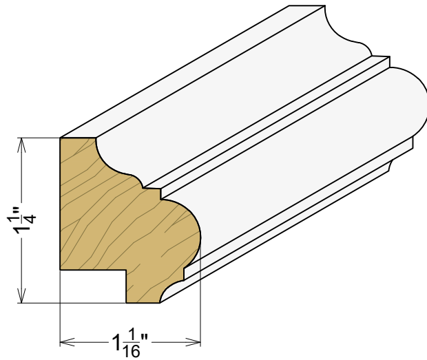
AP 6101 1-1/16" x 1-1/4"
