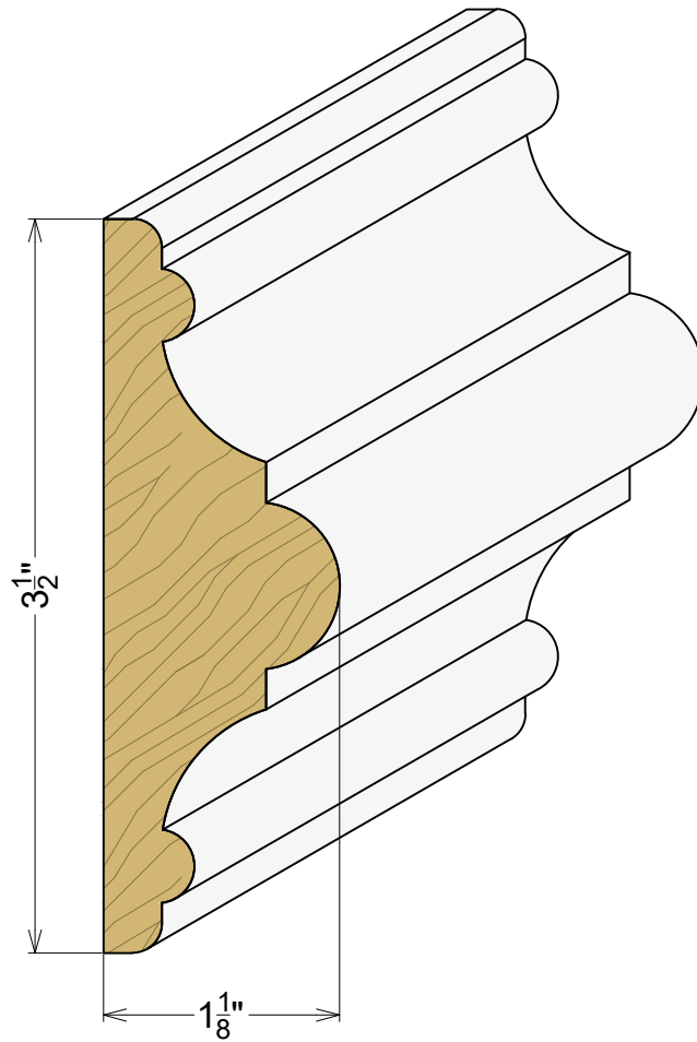
AP 6107 1-1/8" x 3-1/2"
