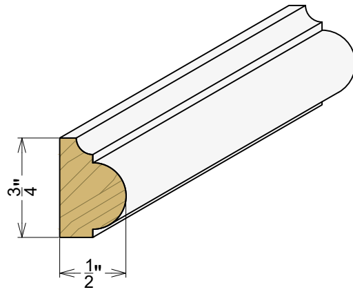
AP 6111 1/2" x 3/4"
