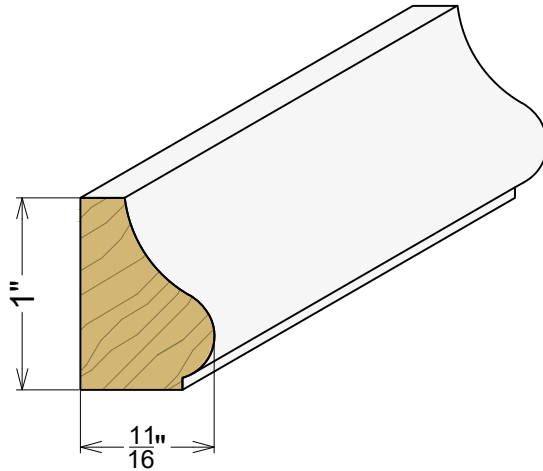
AP 6121 11/16" x 1"
