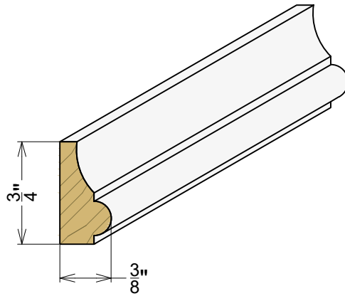
AP 6125 3/8" x 3/4"
