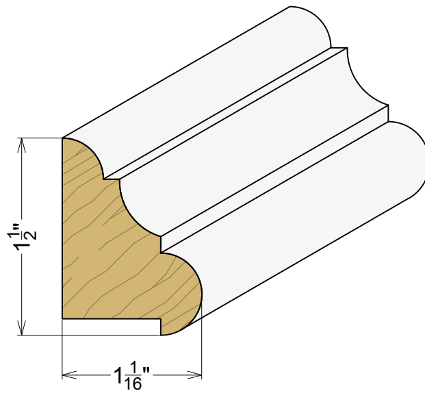
AP 6140 1-1/16" x 1-1/2"
