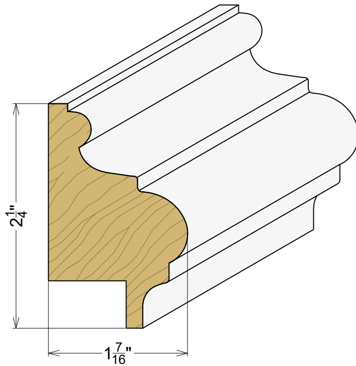
AP 6191 1-7/16" x 2-1/4"
